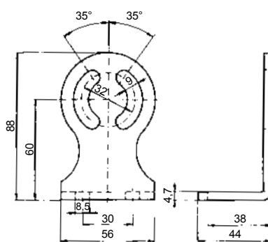
support bracket 02
